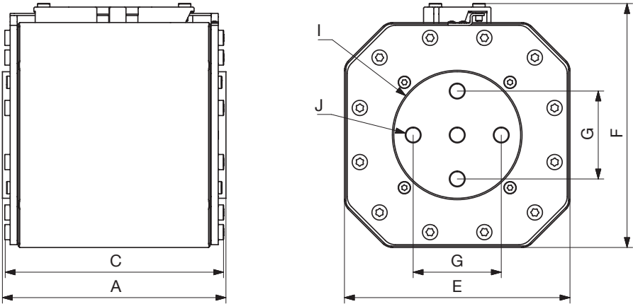
Mounting type 3 : Flush
